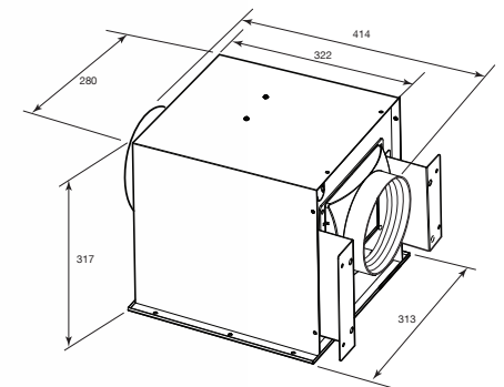
Remote fan motor goes into ceiling space
